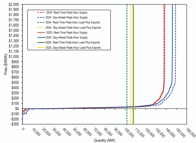
Figure 5 Real-time and day-ahead hourly supply curves: 2024 and 2025
