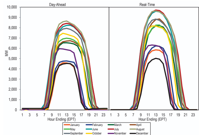
Figure 14 Average hourly real-time generation and day-ahead commitments of solar units: 2025
