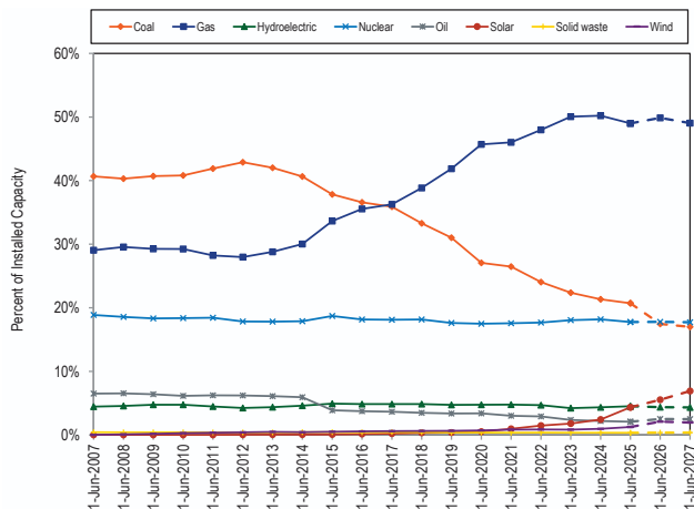
Figure 8 Percent of installed capacity (By fuel source): June 1, 2007 through June 1, 2027
