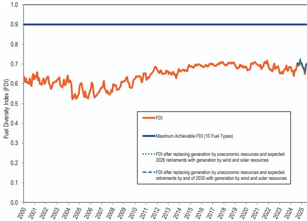
Figure 6 Fuel diversity index for monthly generation: June 2000 through December 2025
