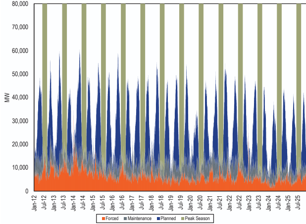
Figure 9 Outages (MW): 2012 through 2025
