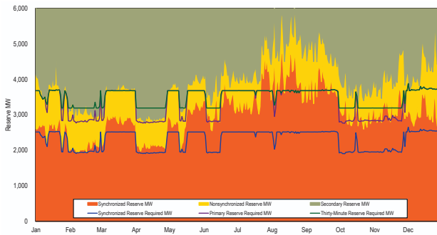
Figure 16 Daily average real-time reserve products cleared and daily average real-time reserve service requirements used by RT SCED: 2025
