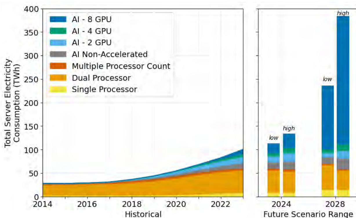
Figure 5.1. Server annual electricity usage by type.
