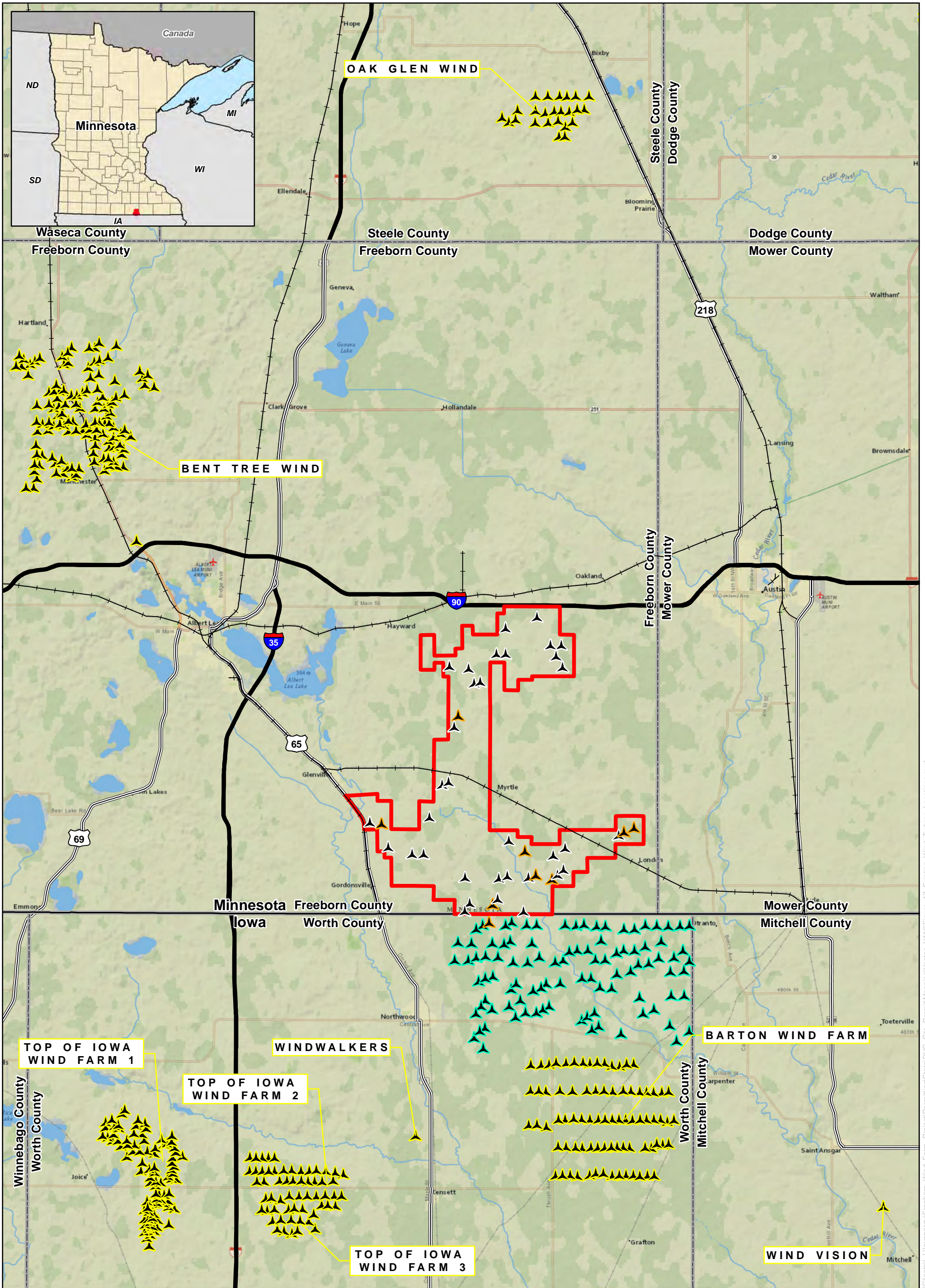
Figure 17 Existing Turbine Locations
