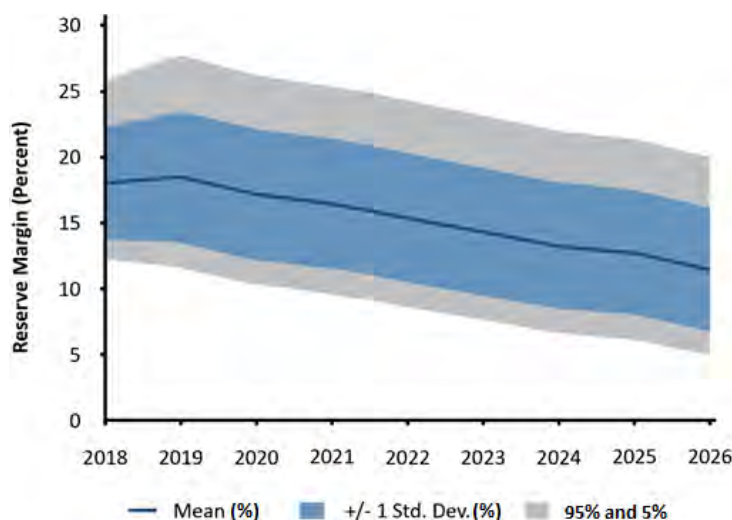
Figure 2.1: Reserve Margin Uncertainty Due to Wind and Solar Variability
