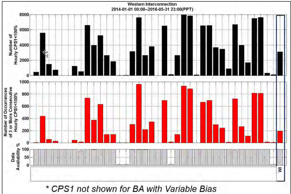
Figure 3.14: Western Interconnection—CPS1 exceedance counts per BA on an hourly basis 39
