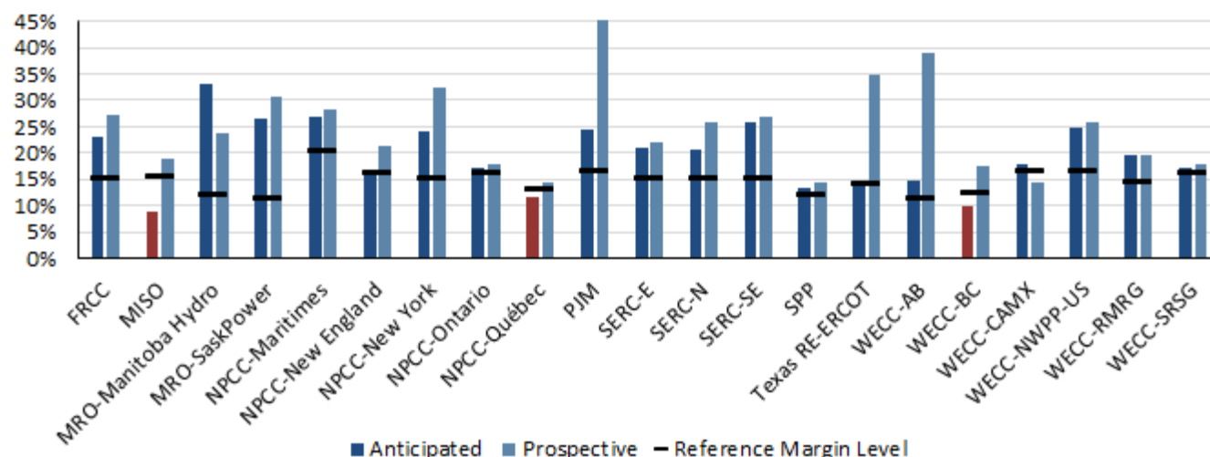
Figure 1.3: Planning Reserve Margins for Year 10 (2026)
