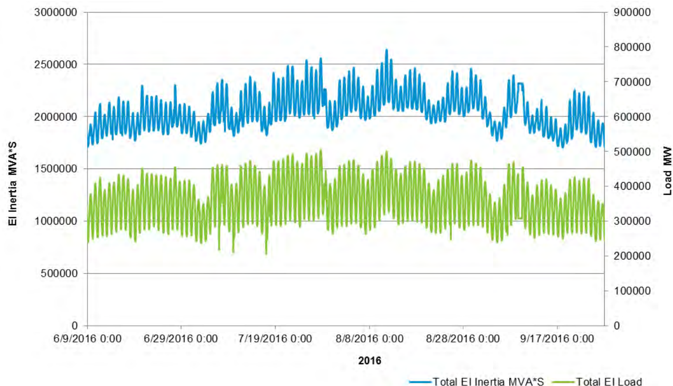
Figure 3.5: Eastern Interconnection System Inertia
