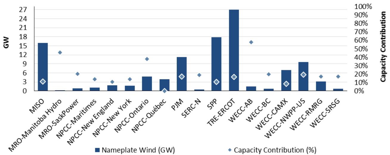
Figure 2.3: 2026 Existing and Tier 1 Wind
