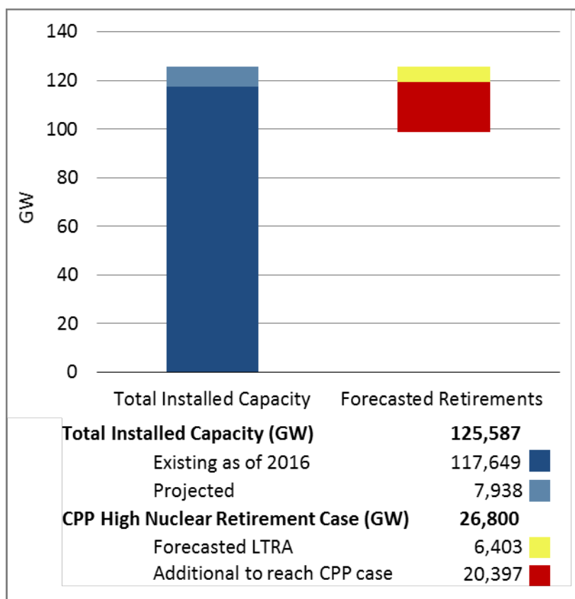
Figure 1.21: Anticipated Nuclear Capacity by 2026
