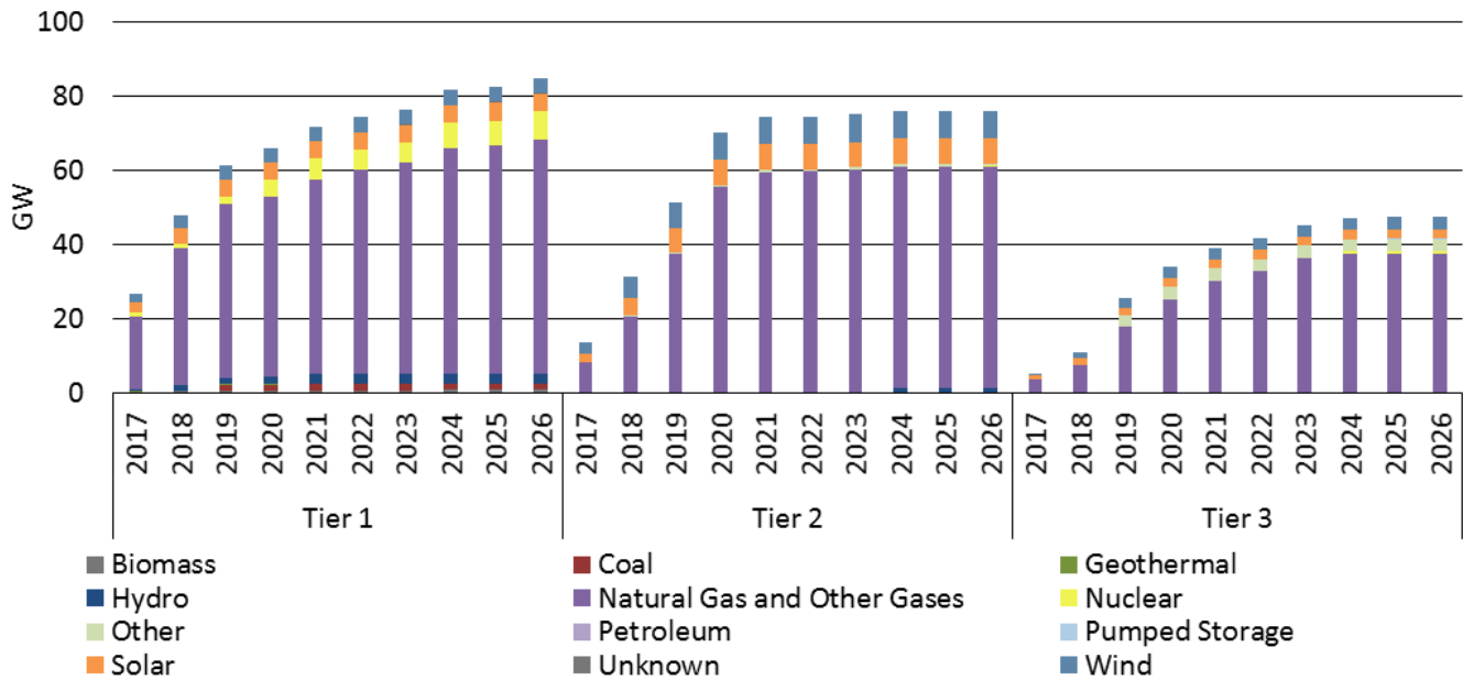
Figure 4.8: Planned Nameplate Capacity Additions by Generation Type and Tier
