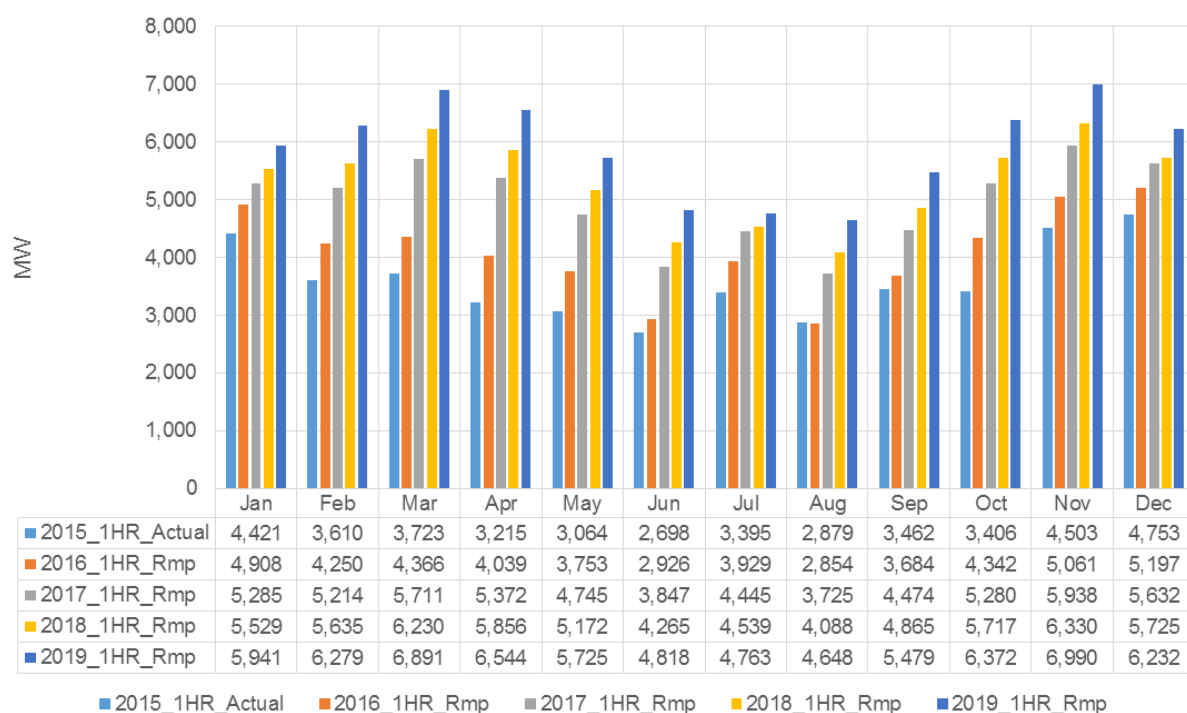
Figure 3.7: CAISO 2015–2019 Monthly One-Hour Upward Ramps
