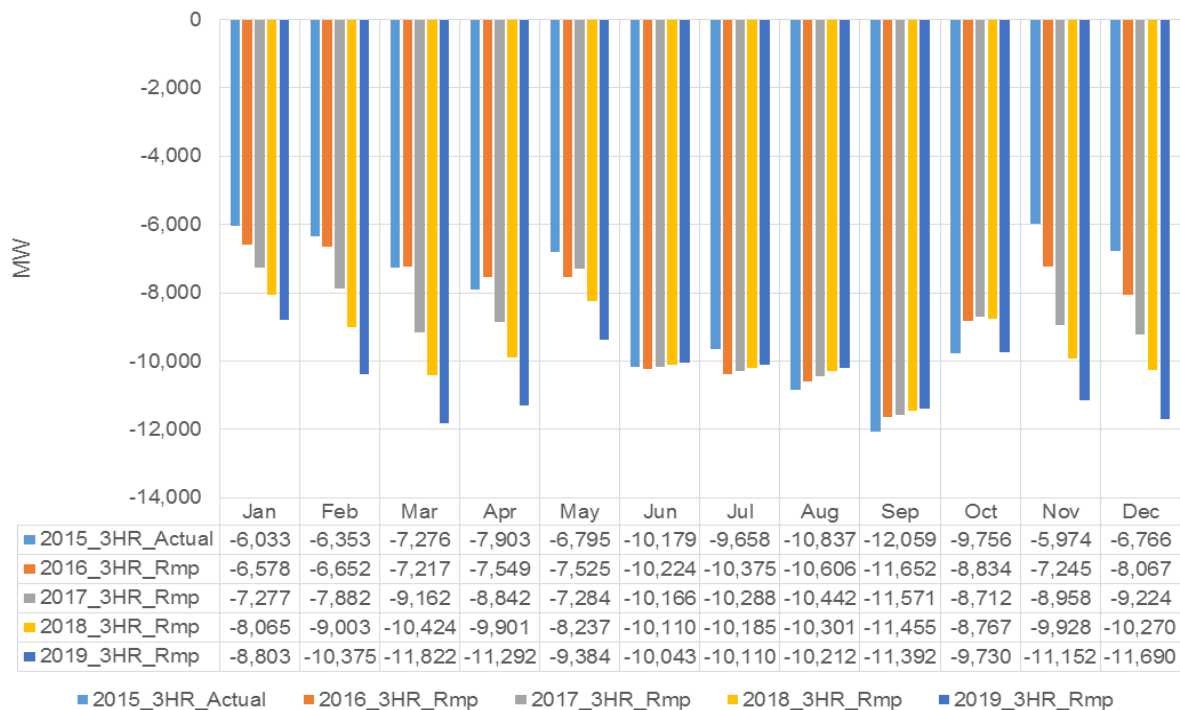
Figure 3.10: CAISO 2015–2019 Monthly Three-Hour Downward Ramps
