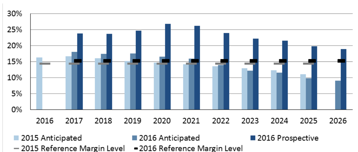
Figure 1.7: MISO 2015 LTRA and 2016 LTRA Reserve Margin Comparison
