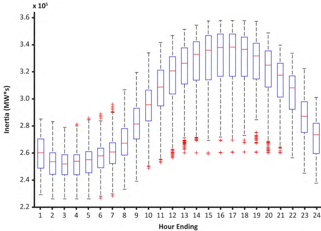
Figure 3.3: ERCOT Inertia by Hour of Day (June 1–July 15 2016)
