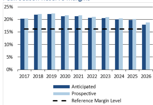
Peak Season Reserve Margins
