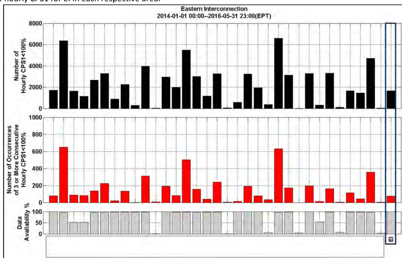
Figure 3.13: Eastern Interconnection—CPS1 exceedance counts per BA on an hourly basis
