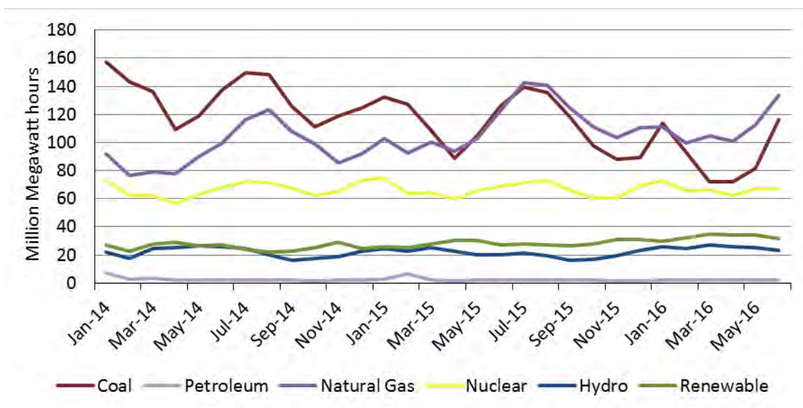
Figure 1.16: Monthly Net Electricity Generation by Fuel Type
