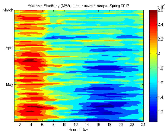
Figure 3.12: ERCOT's Available Flexibility for One Hour Ramps in Spring 2017
