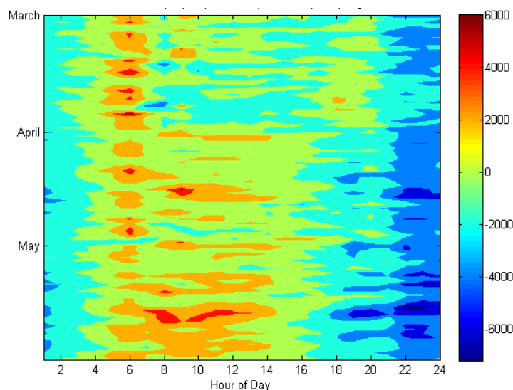
Figure 3.11: ERCOT's Net Load One Hour Ramps for Spring 2017
