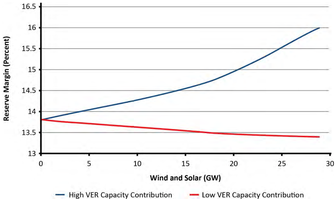
Figure 2.5: Reference Margin Level Increases with Added VER
