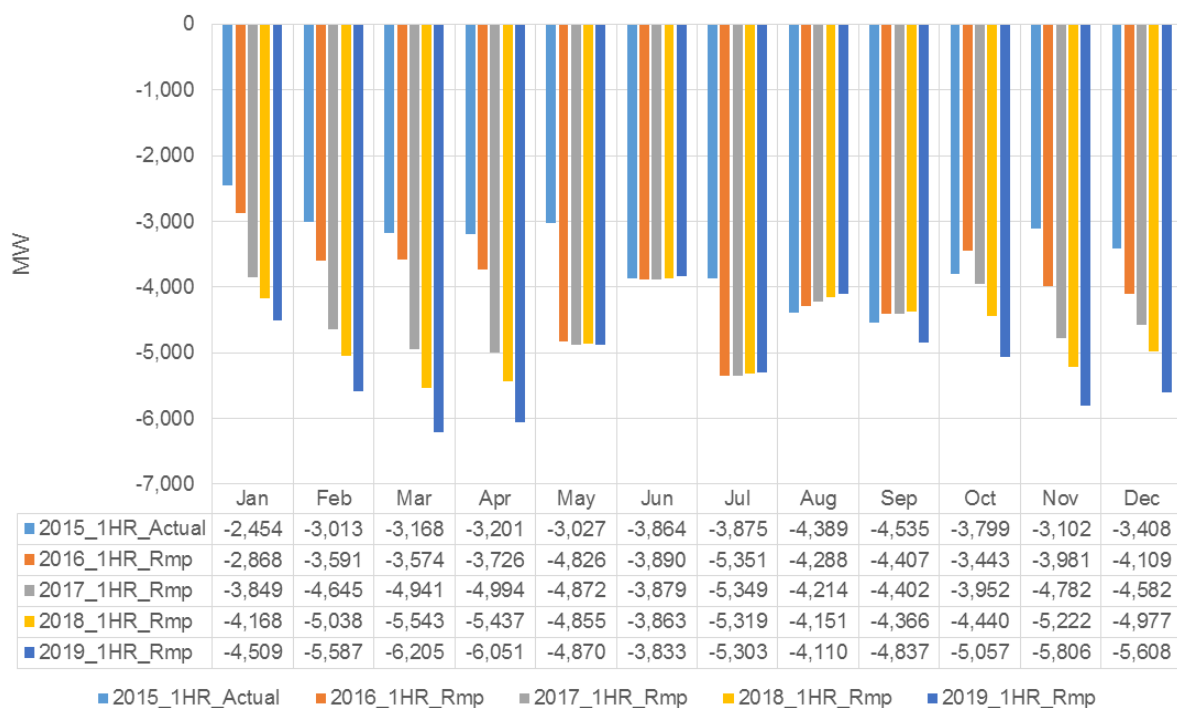
Figure 3.8: CAISO 2015–2019 Monthly One-Hour Downward Ramps
