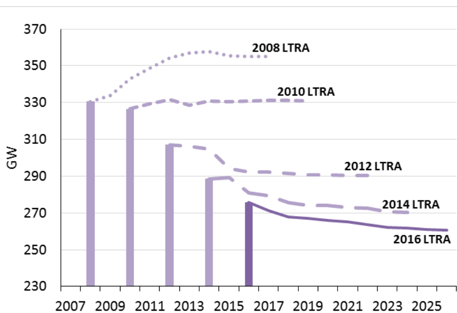
Figure 1.18: Anticipated Coal Capacity by LTRA Reporting Year
