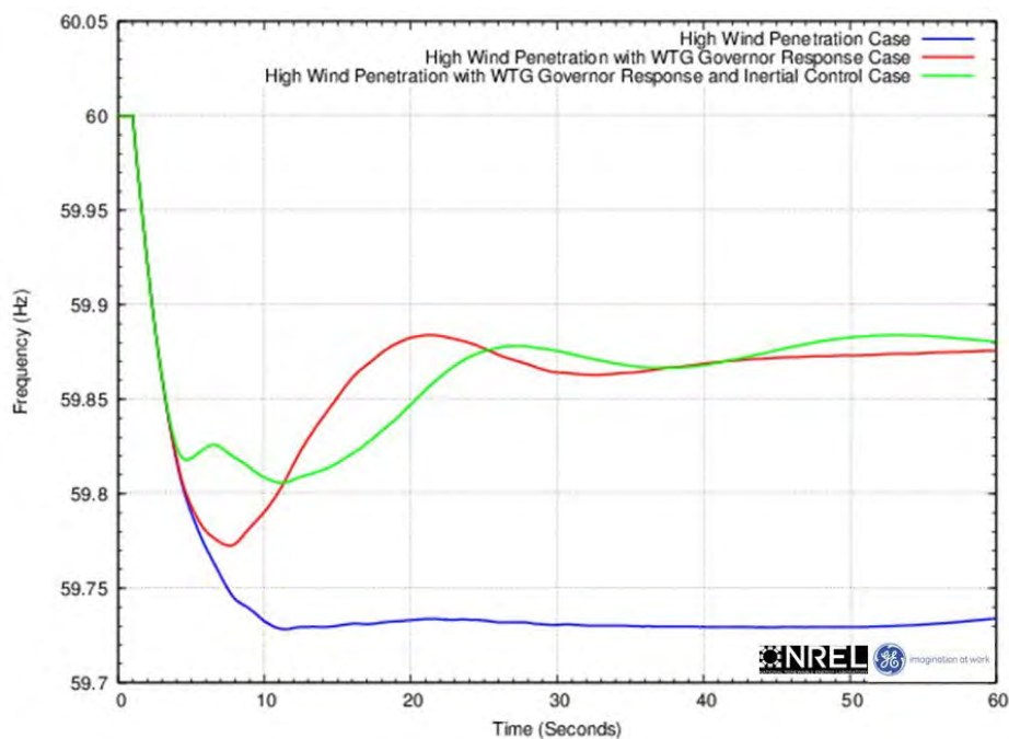
Figure 5.2: Illustration of Wind Turbine Frequency Controls 69
