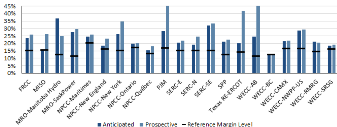
Figure 1.2: Planning Reserve Margins for Year 5 (2021)
