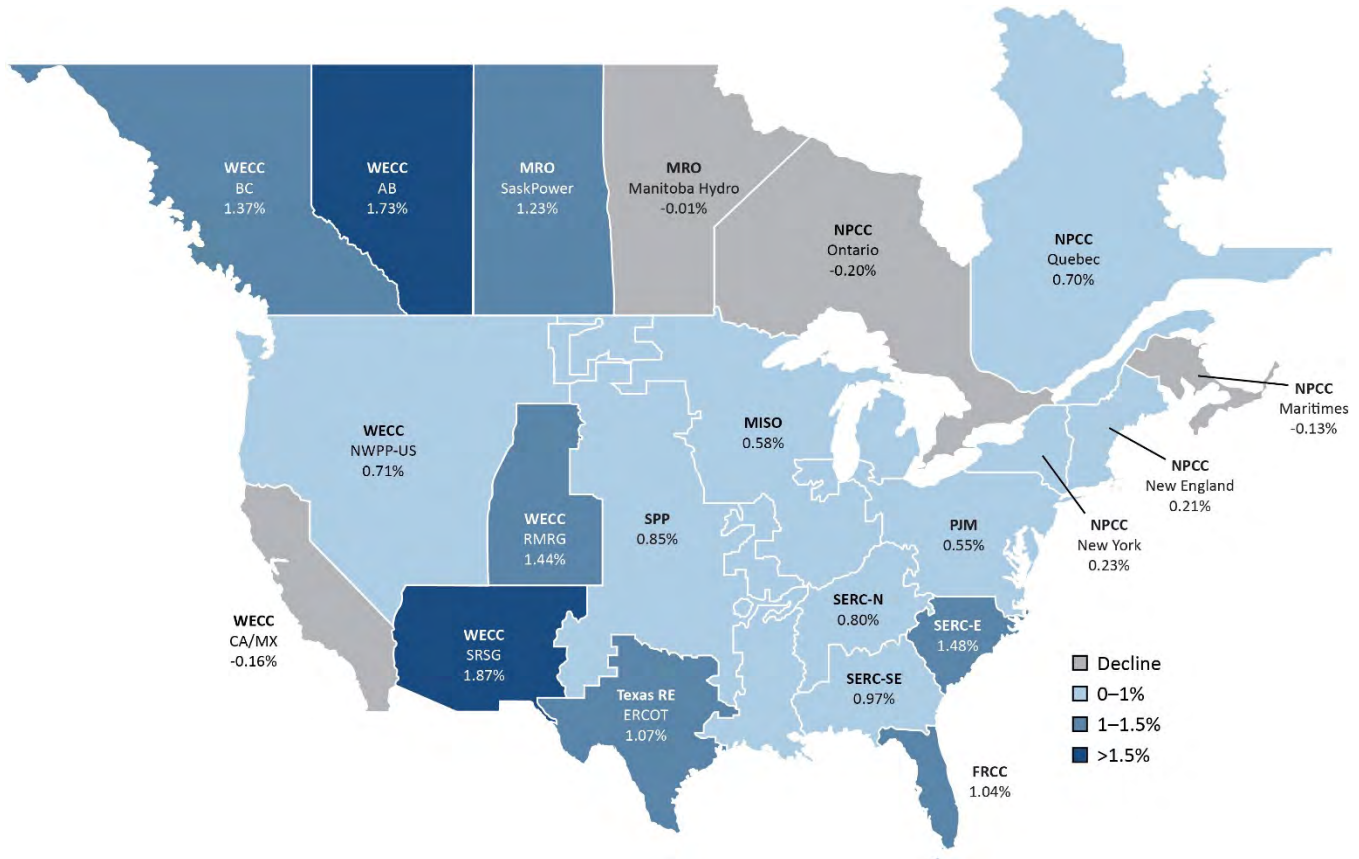
Figure 4.3: GR-Map: Compound Annual Growth Rate by Assessment Area–Demand
