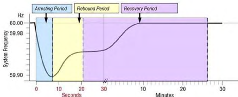
Figure 5.1: Time Frames of Frequency Response
