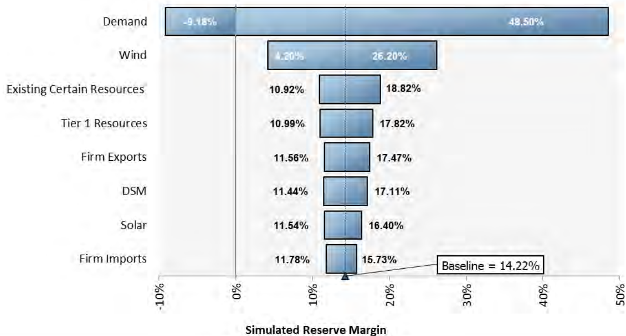
Figure 2.2: Tornado Plot for 2016 Simulated Reserve Margin Ranked by Effect of the Reserve Margin's Mean
