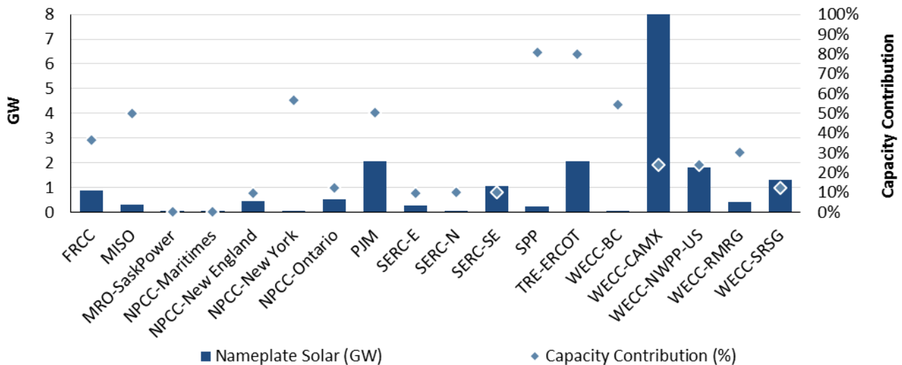
Figure 2.4: 2026 Existing and Tier 1 Solar
