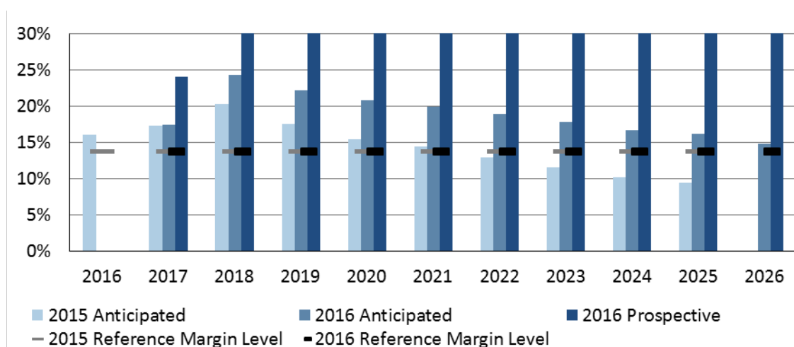
Figure 1.10: Texas RE-ERCOT 2015 LTRA and 2016 LTRA Reserve Margin Comparison
