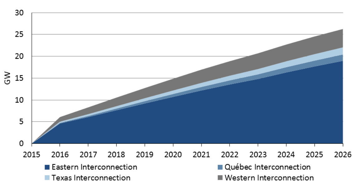
Figure 4.5: Energy Efficiency Projections by Interconnection through 2026
