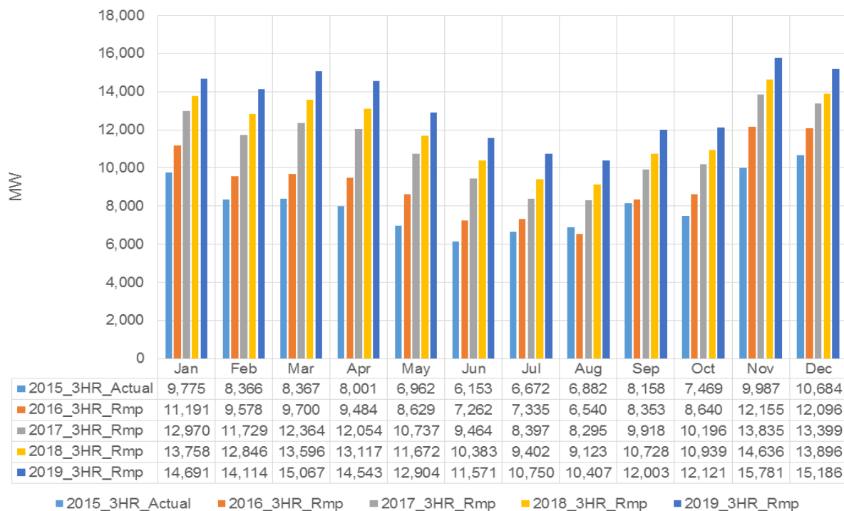
Figure 3.9: CAISO 2015–2019 Monthly Three-Hour Upward Ramps
