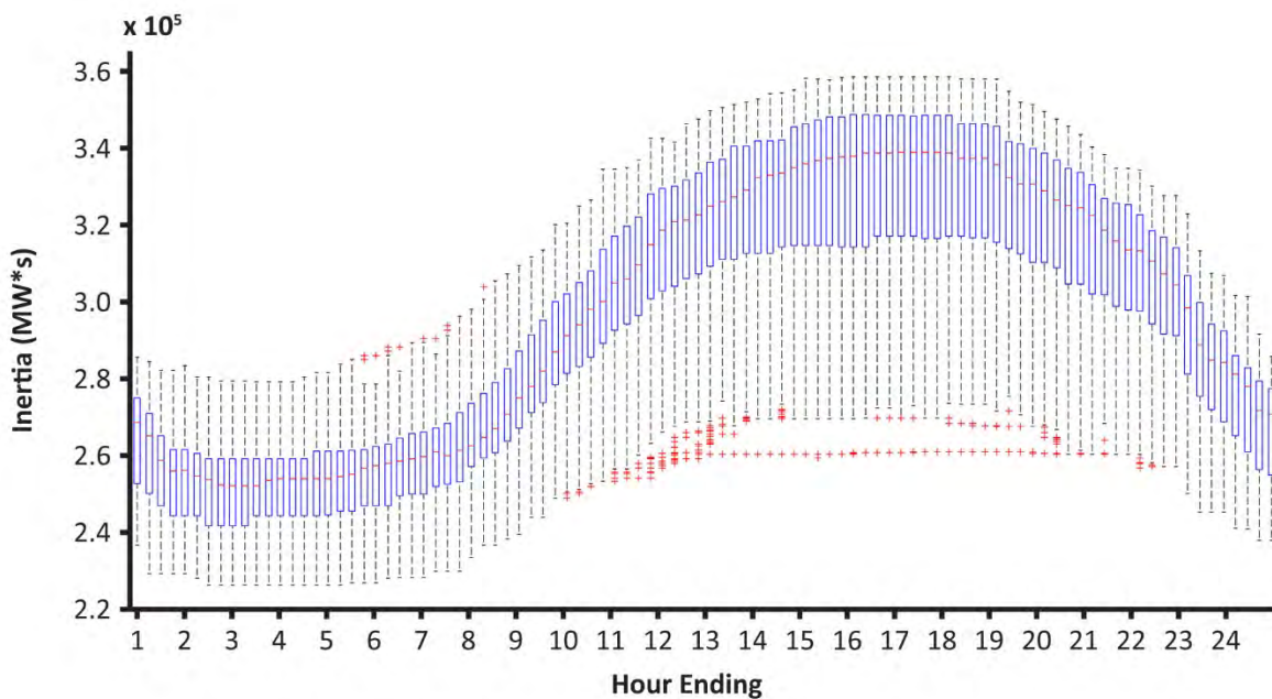
Figure 3.4: ERCOT Inertia by 15-minute Interval of Day (June 1–July 15 2016)
