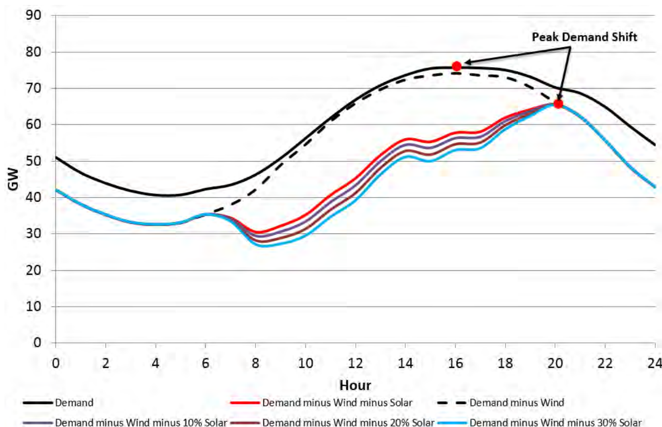
Figure 3.16: Demand and Net Demand Shapes at Different DER Penetration Levels
