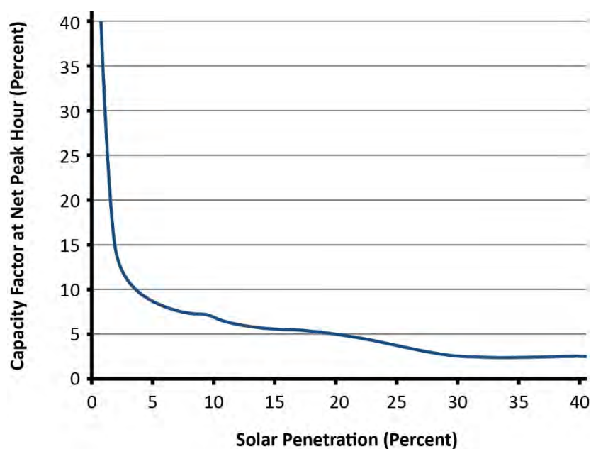
Figure 3.17: Solar Power Capacity Factor
