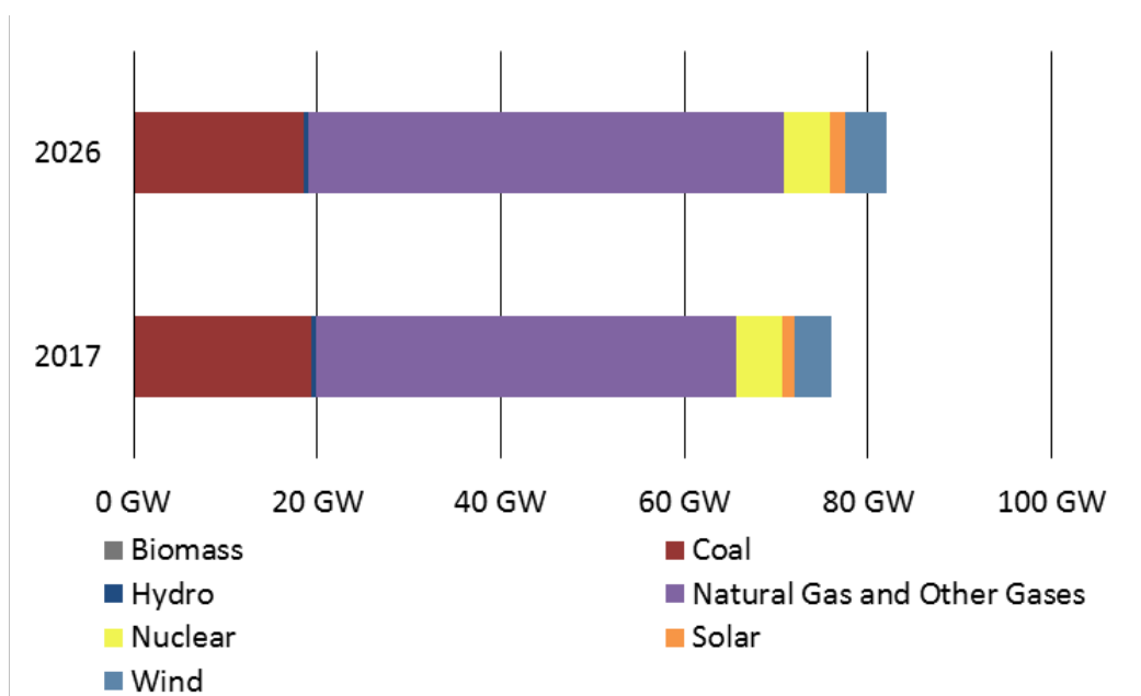
Figure 1.13: ERCOT Total Anticipated Capacity by Fuel Type
