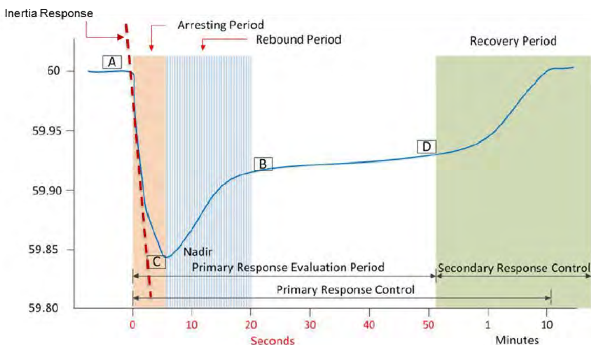
Figure 3.1: Typical Frequency Excursion and Recovery
