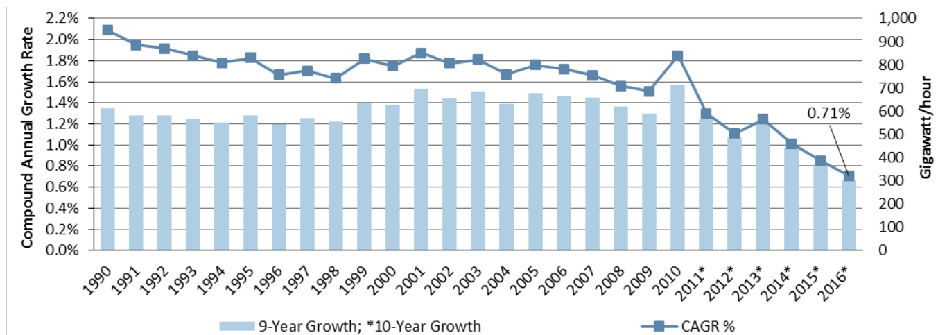
Figure 4.2: Compound Annual Growth Rate–Energy 44
