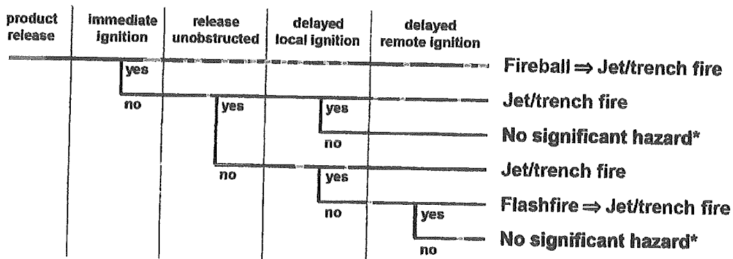
Figure 1.1 Event tree for high pressure gas pipeline failure (adapted from Bilo and Kinsman 1997).
