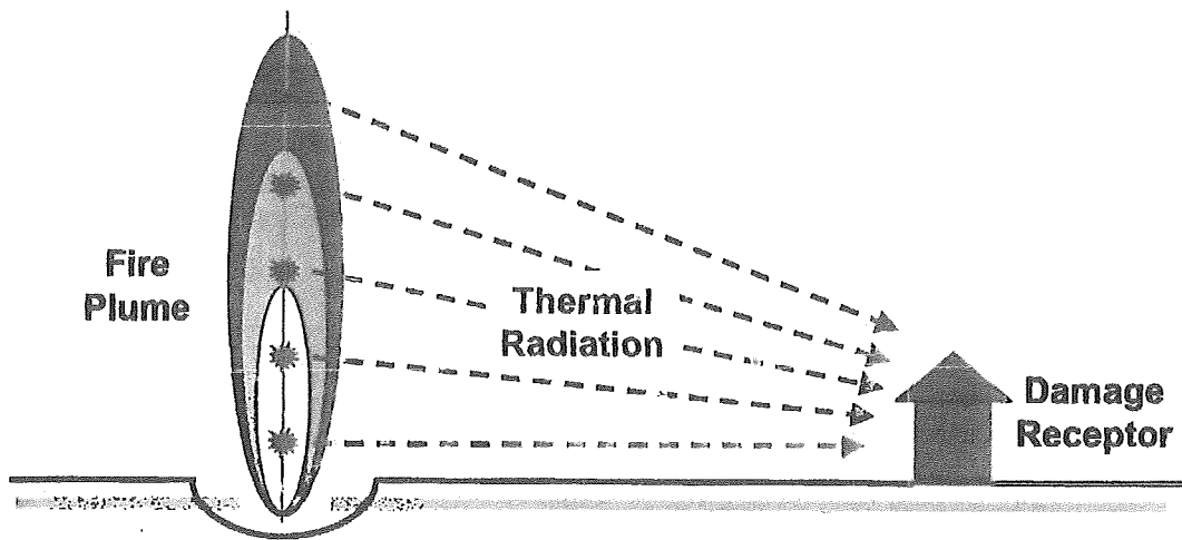
Figure 2.1 Conceptual fire hazard model.
