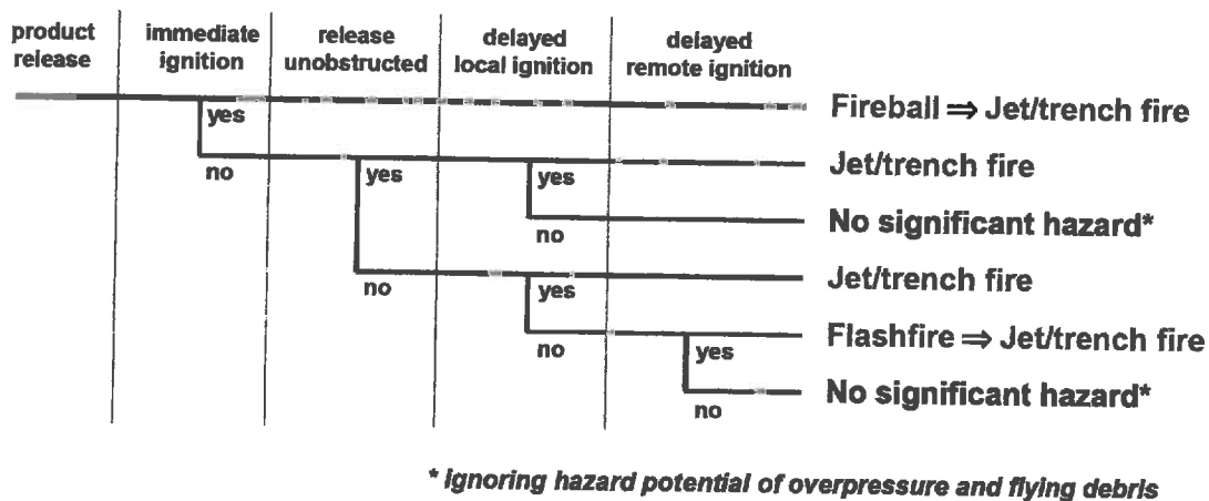
Figure 1.1 Event tree for high pressure gas pipeline failure (adapted from Bilo and Kinsman 1997).
