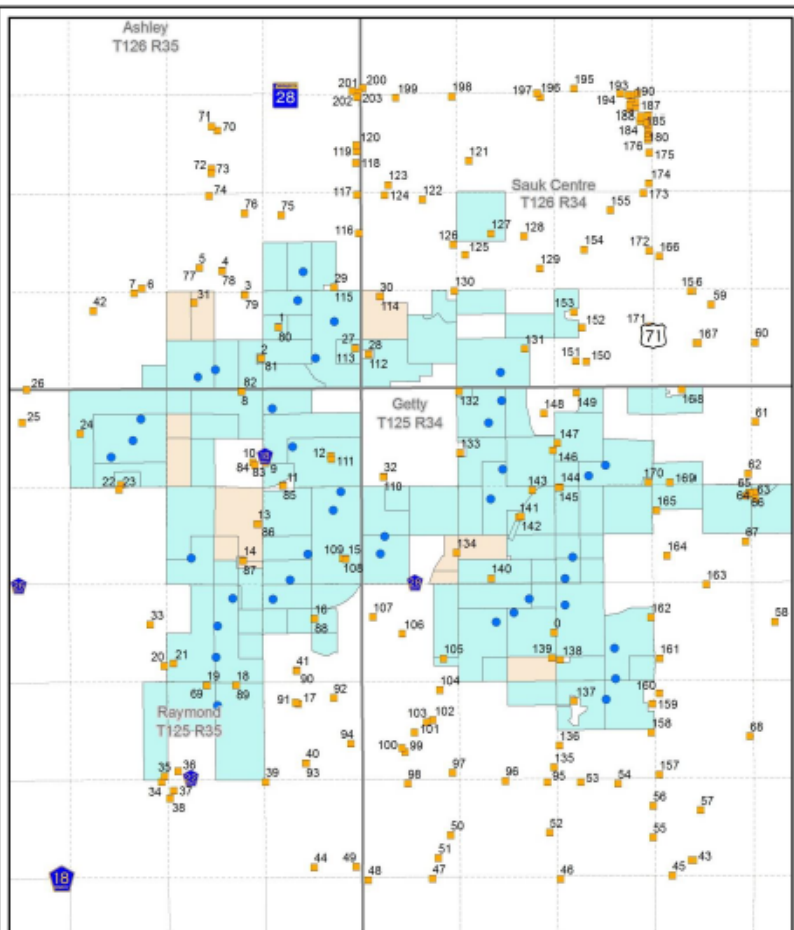
Figure 1. Modeled Residences and Project Turbines
