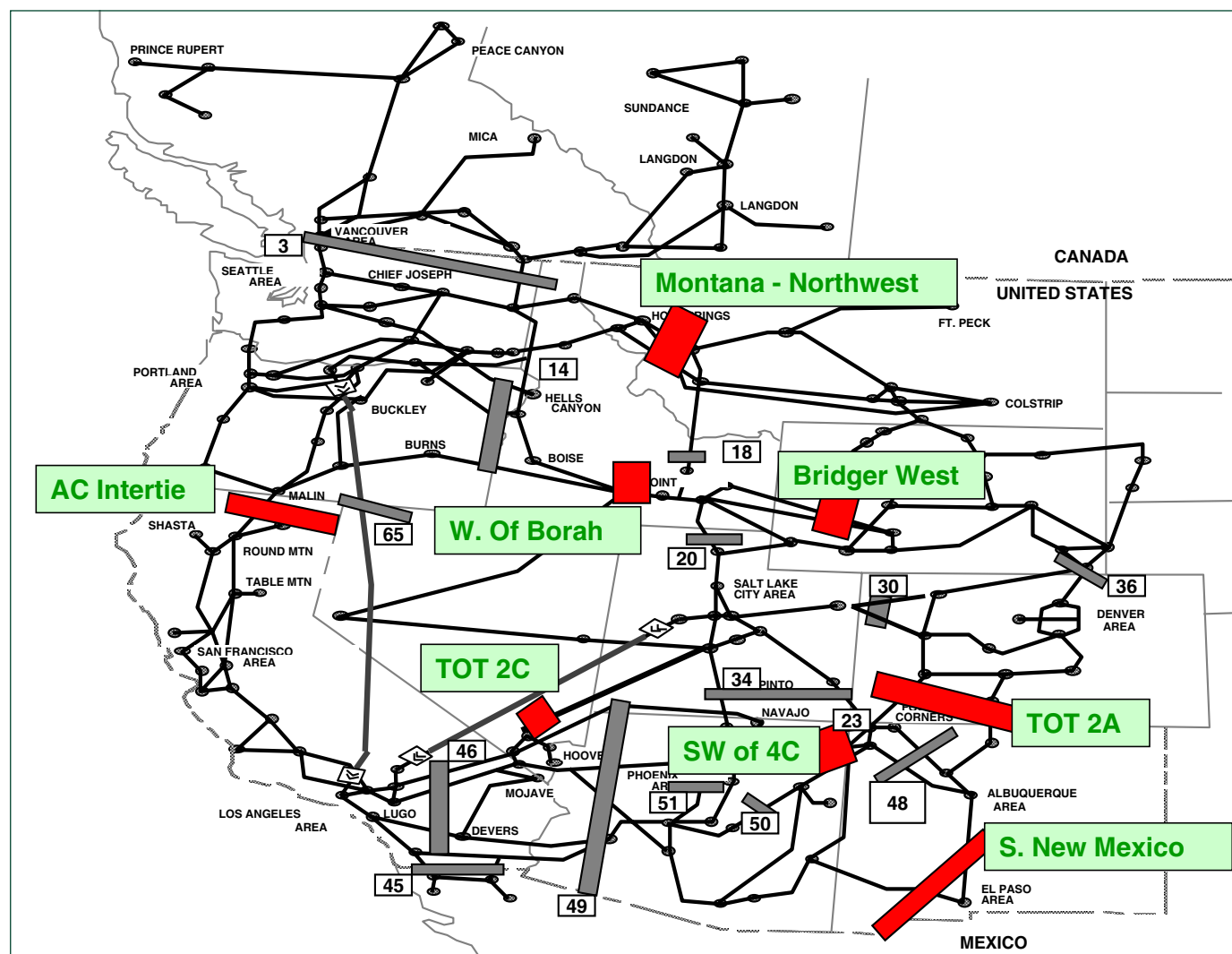
Figure 5-3. Most Heavily Used Transmission Paths in WECC, 2007
