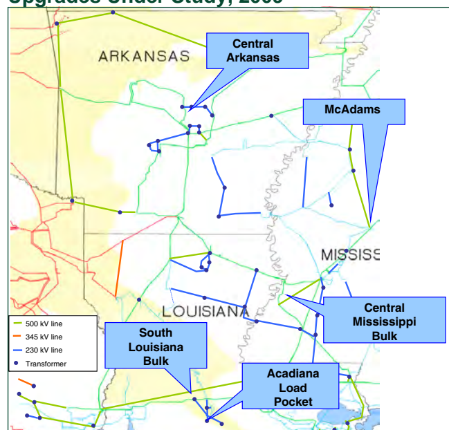
Figure 4-20. Entergy Region Transmission Upgrades Under Study, 2009
