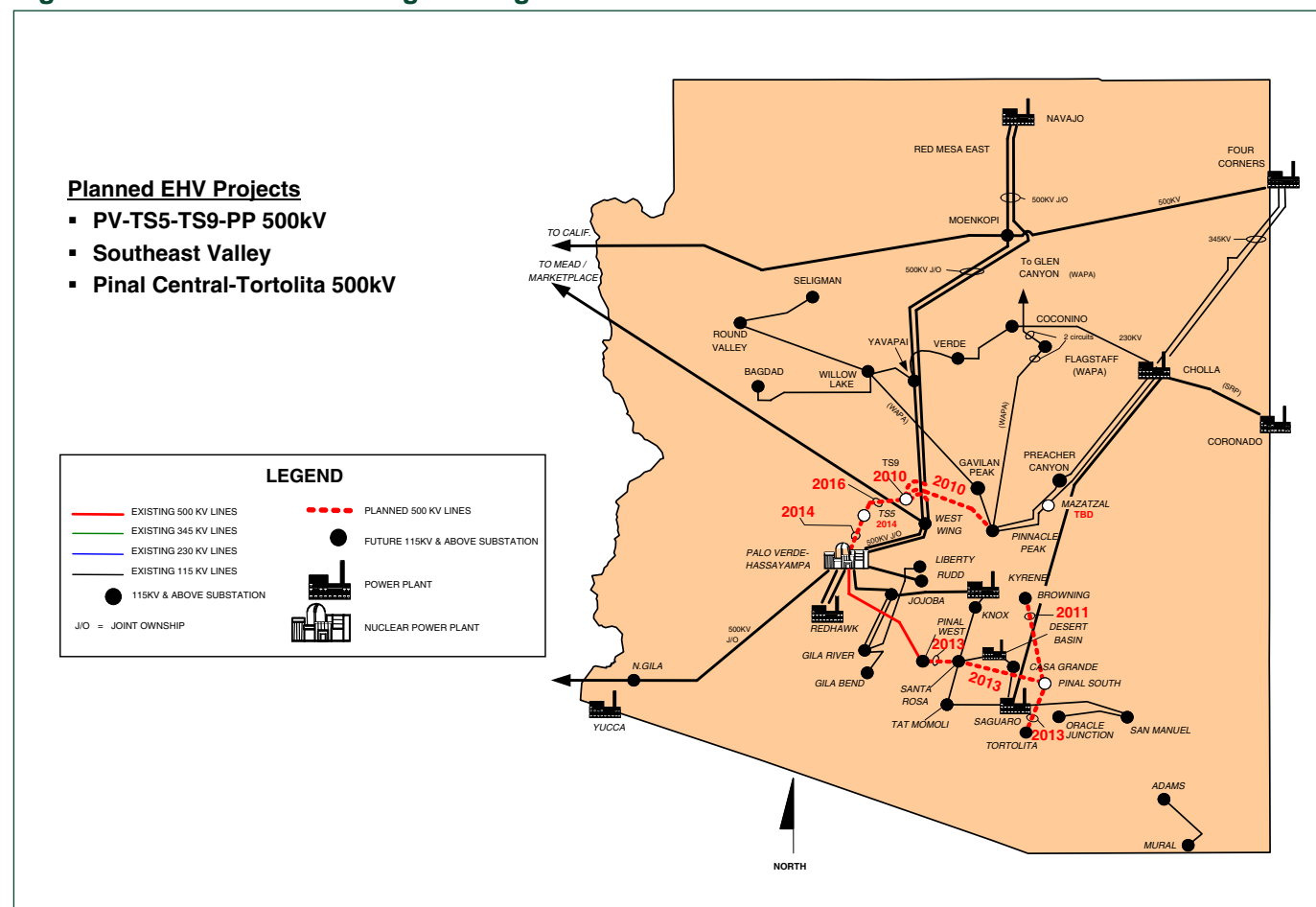
Figure 5-14. Planned Extra High Voltage Transmission Facilities for the Phoenix and Tucson Area
