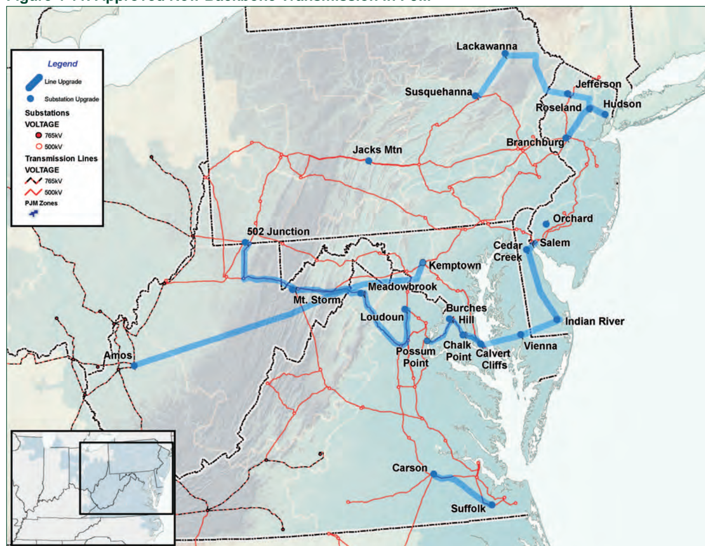
Figure 4-11. Approved New Backbone Transmission in PJM
