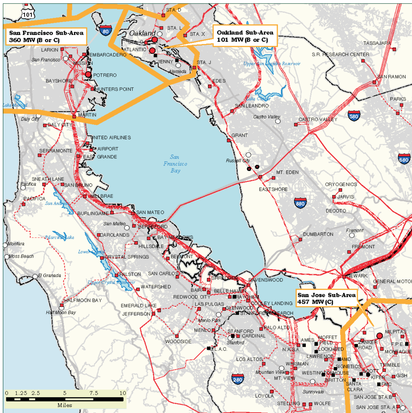
Figure 5-11. Electric System of the Greater San Francisco Bay Area
