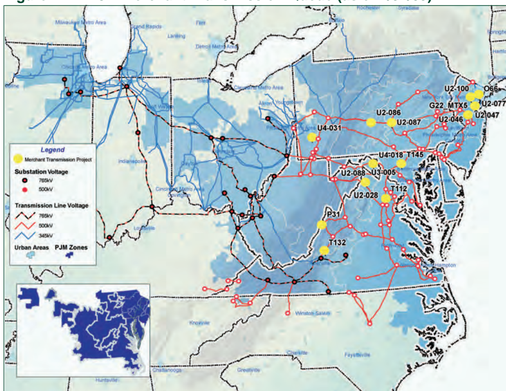
Figure 4-12. PJM Merchant Transmission Queue (as of 1/31/09)
